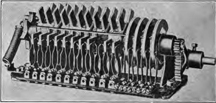
FIG. 309.—A Typical Electrical Vehicle Controller, or Circuit-changing Switch. The circuit terminals of battery and motors are shown at the jack-springs, which are arranged to be engaged by the fins on the periphery of the controller-cylinder. The connections within the controller, between the fins, are the same as those shown in Fig. 308, except for the fact that the four rings at the right hand end provide constant voltage connections for use with a shunt motor. The gaps at the rear of the rings show means for cutting out the shunt field at top speed.
